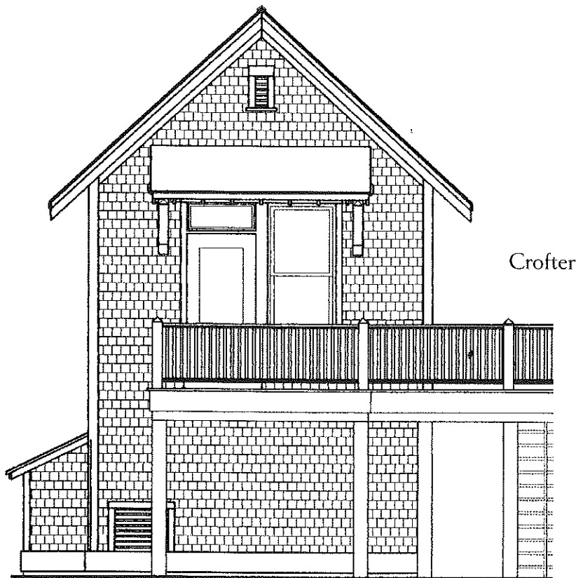
Crofter-garage entry elevation
